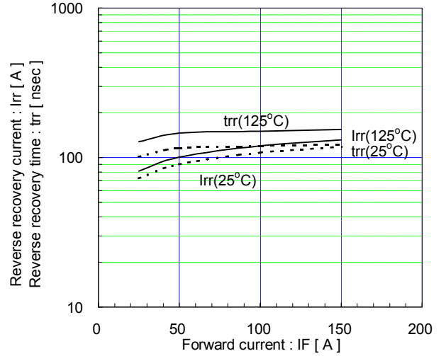
Reverse recovery characteristics (typ.) Vcc=600V, VGE=±15V, RG=5.6Ω
