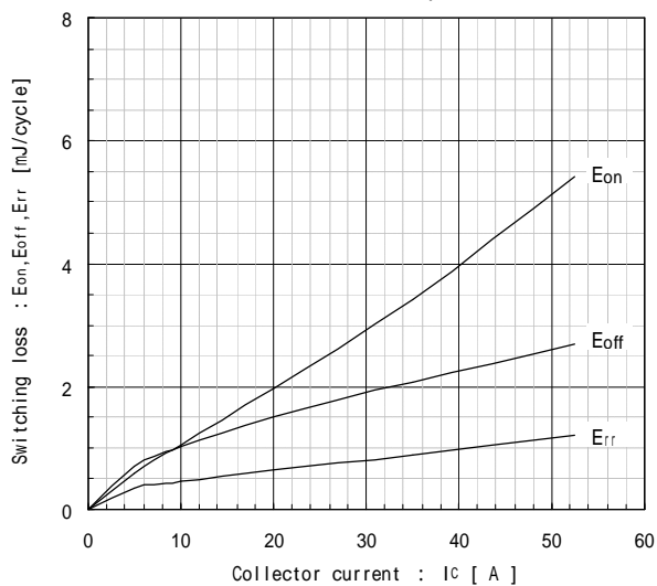
Switching Loss vs. Collector Current (typ.) V_{DC}=600V, V_{CC}=15V, T_j=25
