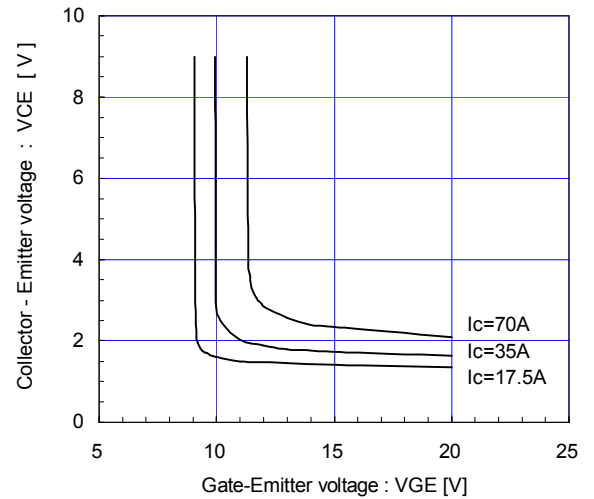
[ Brake ] Collector-Emitter voltage vs. Gate-Emitter voltage (typ.) T_j = 25^\circ\text{C} / chip
