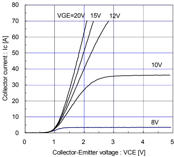
[ Brake ] Collector current vs. Collector-Emitter voltage (typ.) T_j = 25^\circ\text{C} / chip
