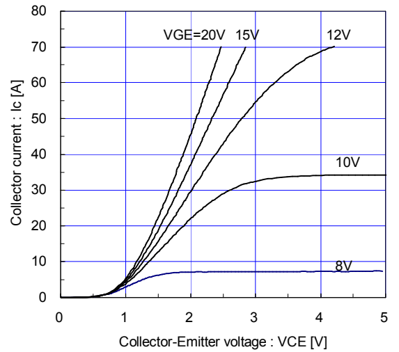
[ Brake ] Collector current vs. Collector-Emitter voltage (typ.) T_j = 125^\circ\text{C} / chip
