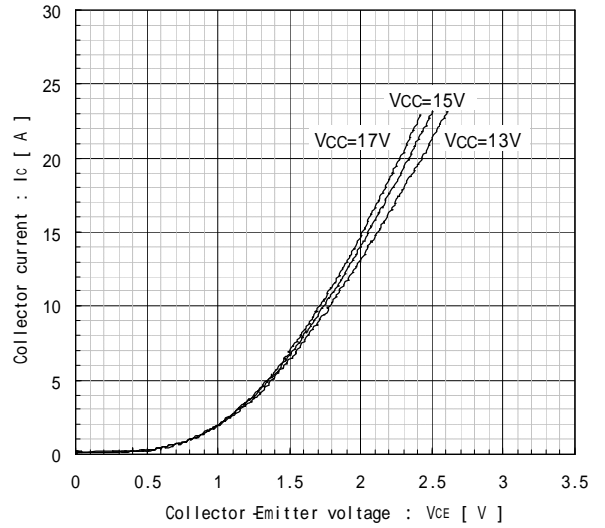
Collector current vs. Collector-Emittor voltage T j =125 [Terminal] (typ.)
