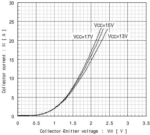
Collector current vs. Collector-Emittor voltage T j =125 [Chip] (typ.)
