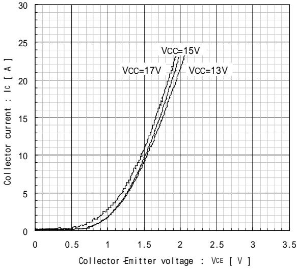
Collector current vs. Collector-Emittor voltage T j =25 [Chip] (typ.)
