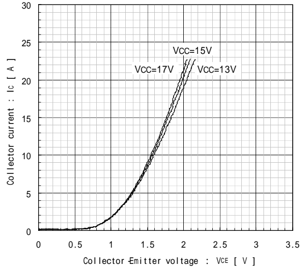
Collector current vs. Collector-Emittor voltage T j =25 [Terminal] (typ.)
