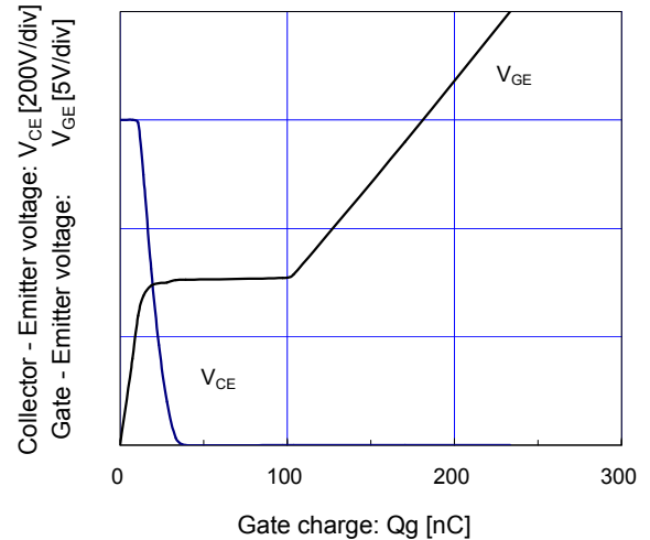
[ Brake ] Dynamic gate charge (typ.) V_{CC} = 600\text{V}, I_c = 25\text{A}, T_j = 25^\circ\text{C}
