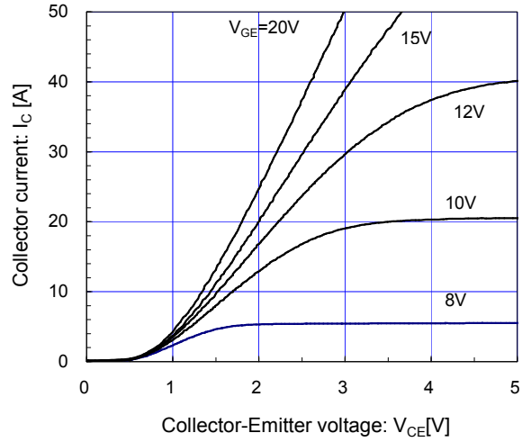
[ Brake ] Collector current vs. Collector-Emittor voltage (typ.) T_j = 150^\circ\text{C} / \text{chip}
