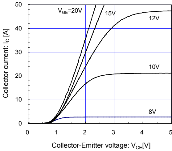
[ Brake ] Collector current vs. Collector-Emittor voltage (typ.) T_j = 25^\circ\text{C} / \text{chip}
