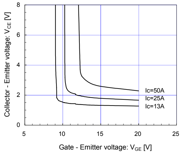
[ Brake ] Collector-Emittor voltage vs. Gate-Emittor voltage (typ.) T_j = 25^\circ\text{C} / \text{chip}
