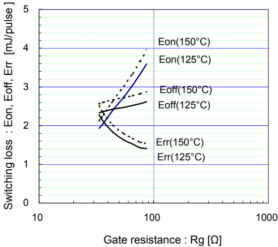
[ Inverter ] Switching loss vs. gate resistance (typ.) V_{CC}=600V, I_c=25A, V_{GE}=\pm 15V
