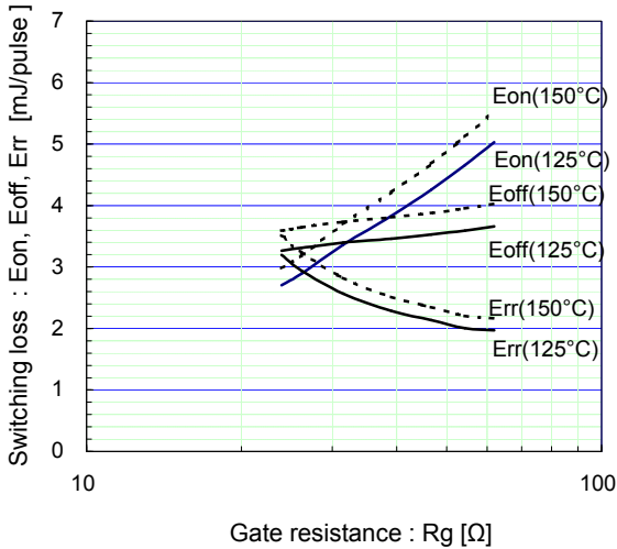
[ Inverter ] Switching loss vs. gate resistance (typ.) V_{CC}=600V, I_C=35A, V_{GE}=\pm 15V
