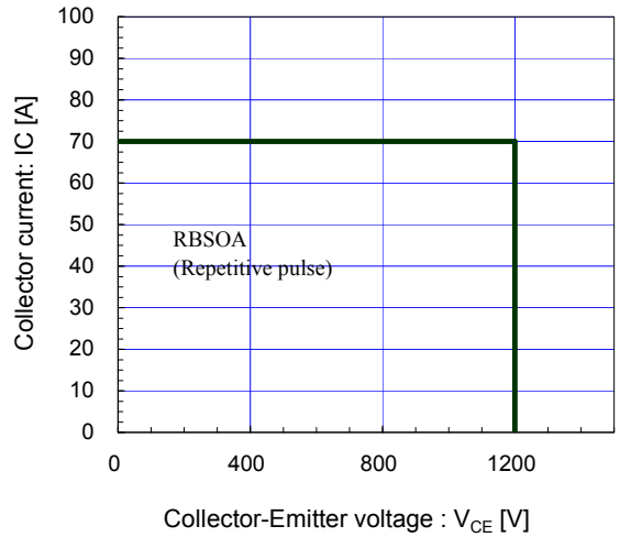
[ Inverter ] Reverse bias safe operating area (max.) +V_{GE}=15V, -V_{GE} \le 15V, R_G \ge 27\Omega, T_J=150^\circ C
