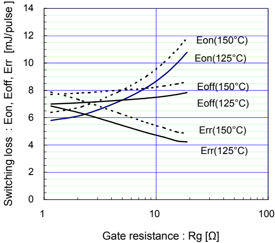
[ Inverter ] Switching Loss vs. gate resistance (typ.) V_{CC}=600V, I_c=75A, V_{GE}=\pm 15V
