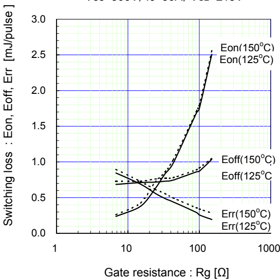
[ Inverter ]
