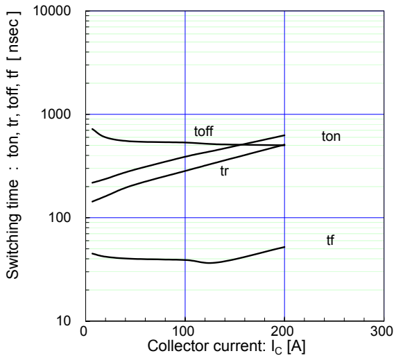
[ Inverter ]
