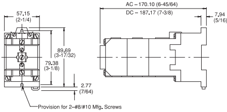
Provision for 2-#8/#10 Mfg. Screws 10- and 12-pole Bulletin 700S-P
