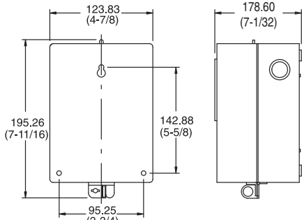
Type 1 Enclosure
