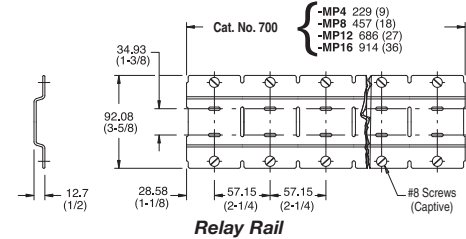
Relay Rail
