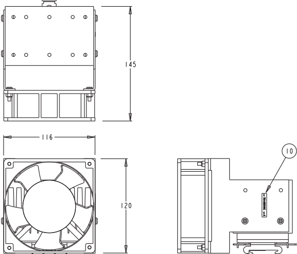
700-SN50VHC
