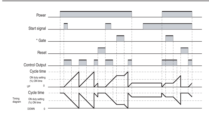
Output Mode S: Stop Watch (Timer resets when power comes ON)
