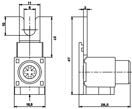
Cat. No. 700-SHTRMA
