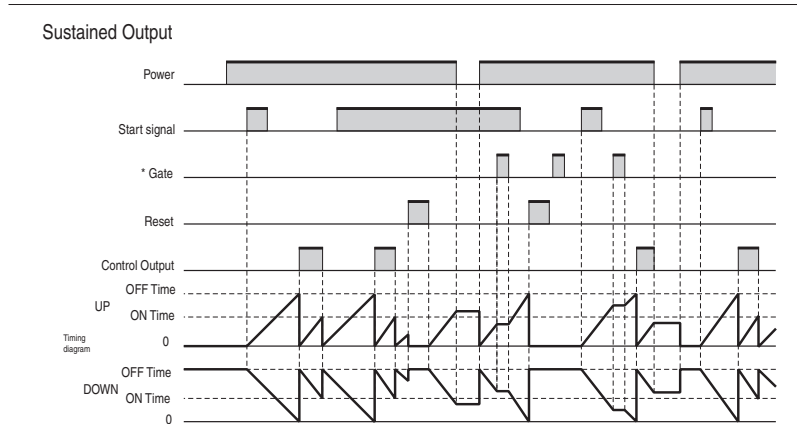
Output Mode T OFF: Twin Timer OFF start
