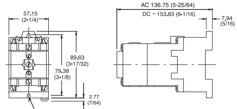
Provision for 2 #8/#10 Mfg. Screws 6- and 8-pole Bulletin 700S-P Relay
