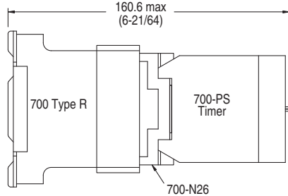
Bulletin 700-PS Timer Mounted on a 4-Pole Bulletin 700-R Relay
