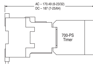
Bulletin 700-PS Timer Mounted on a 4-pole Bulletin 700-P or -PK Relay or 2-pole Bulletin 700-PH Relay Approximate Shipping Weight: AC – 0.68 kg (1.5 lb) without 700-PS, eDC – 1.34 kg (2.9 lb) without 700-PS
