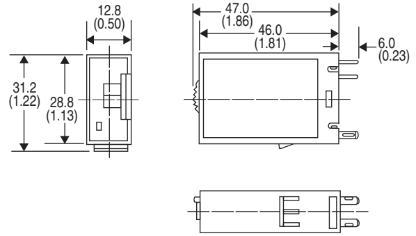
Bulletin 700-HNK42 DPST-NO Contact Approximate Dimensions
