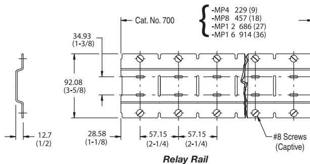
Relay Rail
