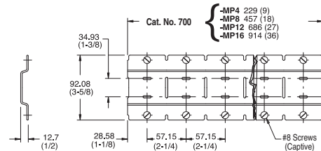
Relay Rail for Bulletin 700-P, -PH, -PK, -N, -NM, -R, -RM, -RT, -RTA Relays Secure the mounting strip with two screws at each end relay position. Use a minimum of one screw at the 3rd, 5th, 7th, etc., relay positions. Alternate between upper and lower horizontal slots.
