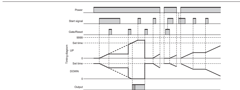
Output Mode S: Stop Watch (Timer resets when power comes ON)
