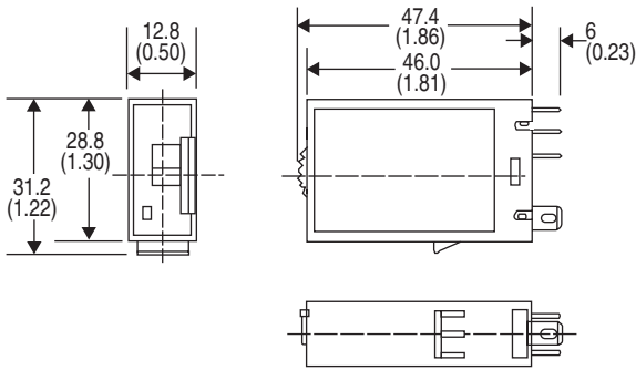
Bulletin 700-HNK41 SPDT Contact Approximate Dimensions
