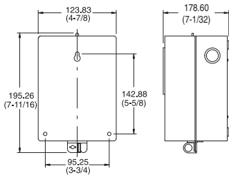
Cat. No. 700-N31, Type 1 Enclosure for Bulletin 700-P, -PH, -PK, -RTC Relays Approximate Shipping Weight: 1.26 kg (2.8 lb)
