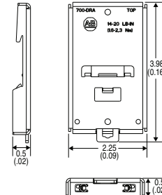
Bulletin 700-R with 852s timer
