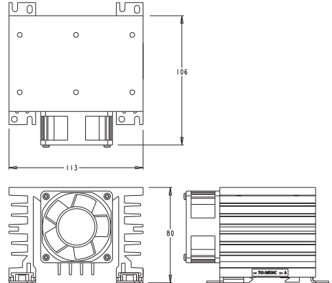
700-SN50HC
