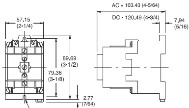
Provision for 2-#8/#10 Mfg. Screws 2- and 4-pole Bulletin 700S-P Relay
