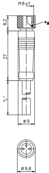
*a O-Ring O-ring
