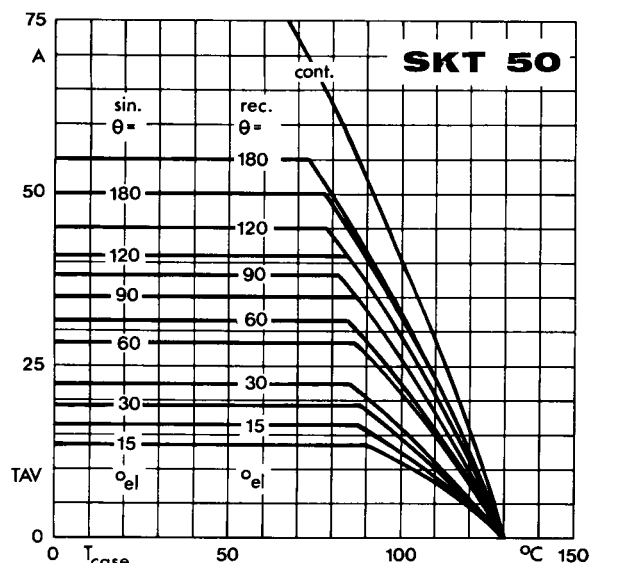
Fig. 2 b Rated on-state current vs. case temperature
