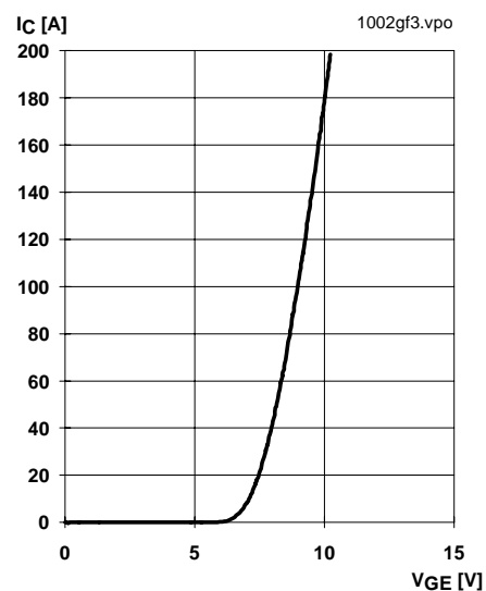
Fig. 12 Typ. transfer characteristic, t_p = 80\text{ }\mu\text{s} ; V_{\text{CE}} = 20\text{ V}
