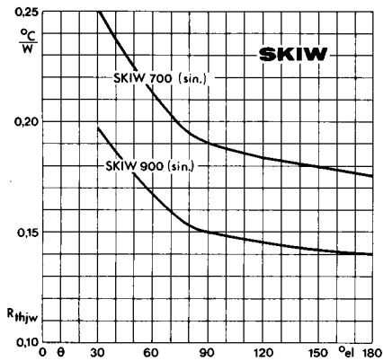
Fig. 6 Thermal resistance vs. conduction angle
