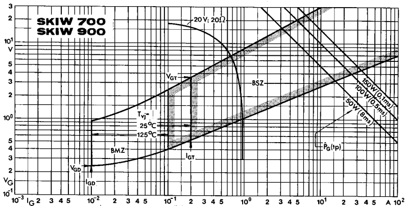
Fig. 8 Gate trigger characteristics
