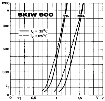
Fig. 5 b On-state characteristics
