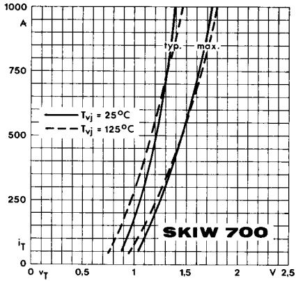
Fig. 5 a On-state characteristics
