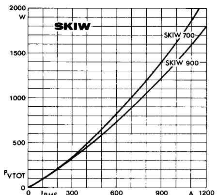
Fig. 4 Power dissipation vs. rms on-state current
