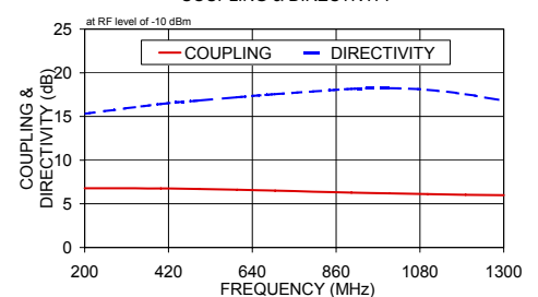
ADC-6-13 COUPLING & DIRECTIVITY
